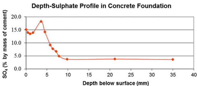
Fig. 22 Typical sulphate profile for in situ cast concrete
