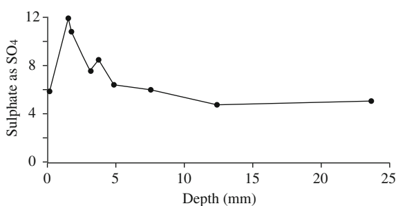
Fig. 33 Relationship between % \text{SO}_4 and distance from top of concrete pier
