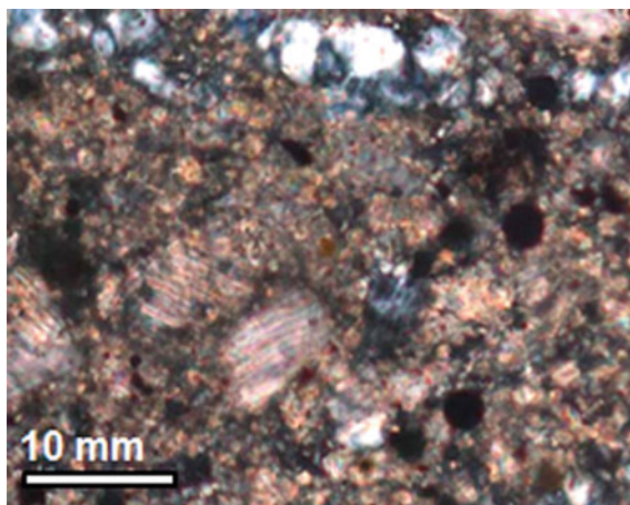
Fig. 63 Oxidised pyrite contained in fragments within concrete aggregate
