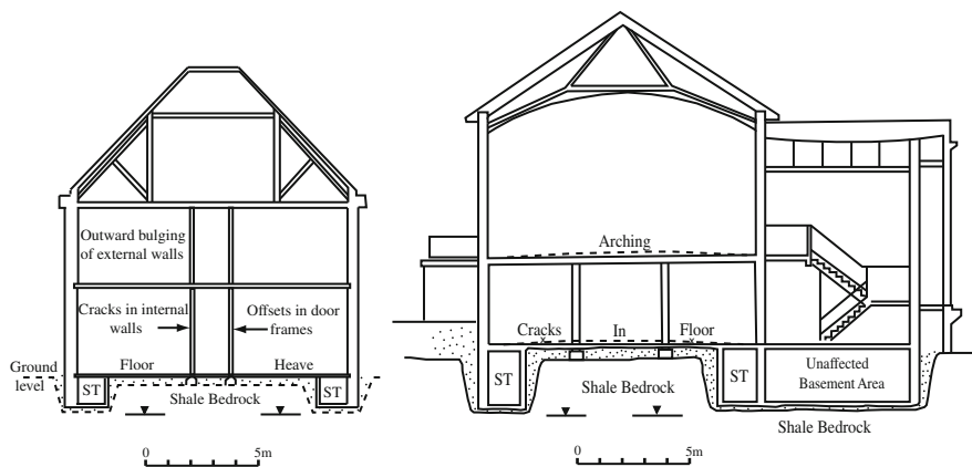
Fig. 44 Similarity between the layout of Llandough Hospital ( left ) and Rideau Health Centre ( right ); ST service tunnels
