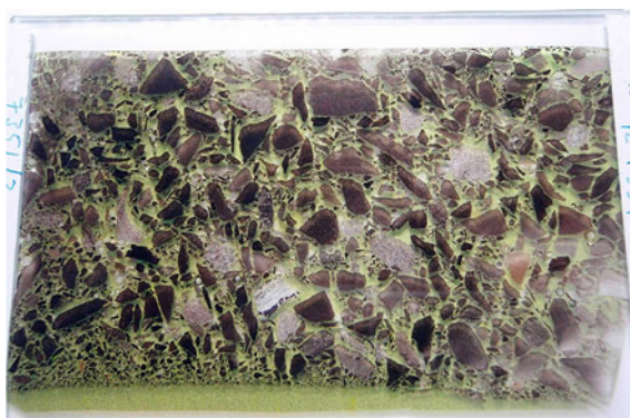
Fig. 4 Petrographic thin section ( 50 \times 70 mm) of an embedded laboratory-crushed fill sub-sample
