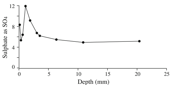
Fig. 35 Relationship between % \text{SO}_4 and distance from concrete surface
