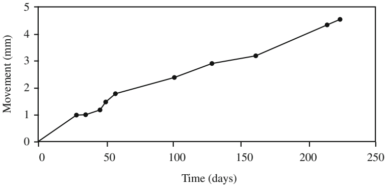
Fig. 70 Levelling of a point on a large reinforced concrete floor slab
