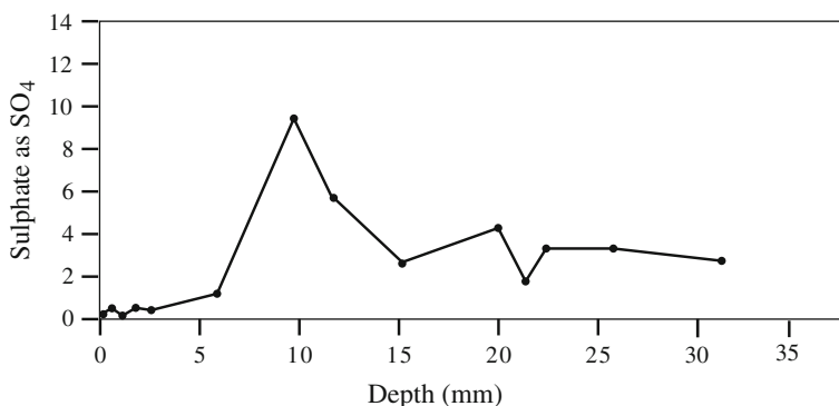
Fig. 18 Variation in sulphate content from the outer surface of the concrete block
