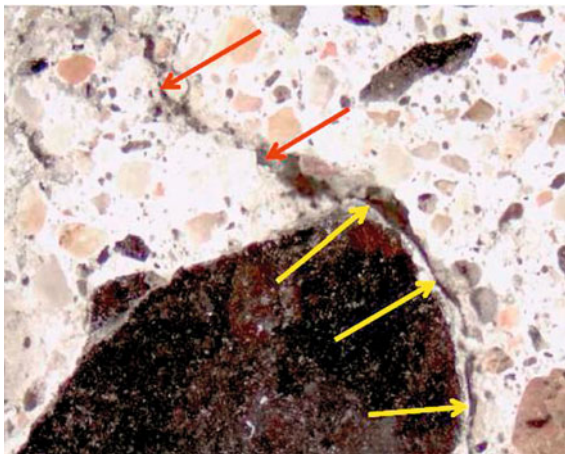
Fig. 21 Photomicrograph showing crack in concrete at coarse aggregate and paste interface
